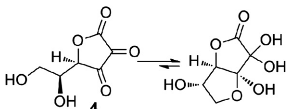
Scheme 2. Reactivity of 4 .
