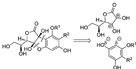
Scheme 1. Retrosynthetic analysis.
